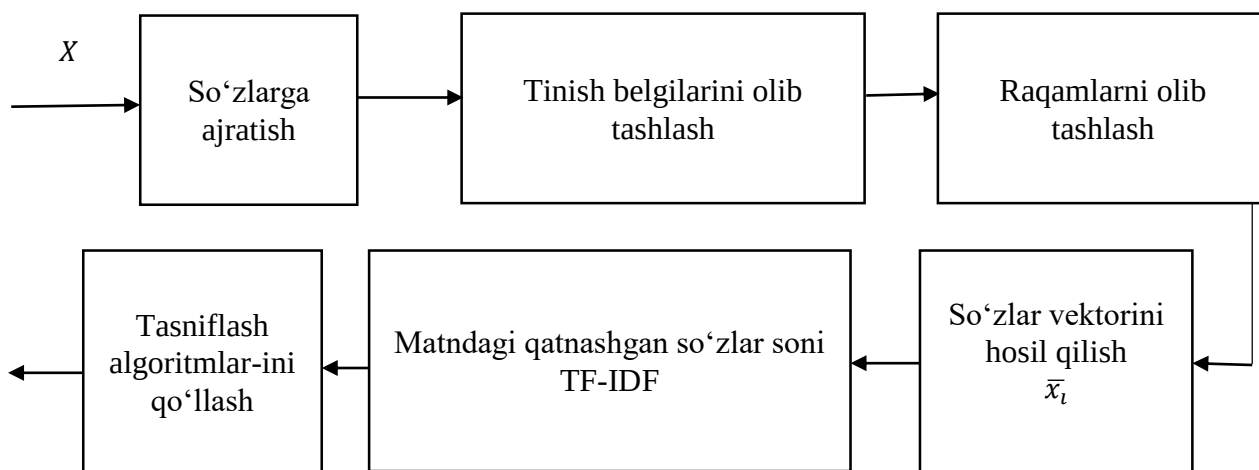
2-rasm. Tasniflash modelini amalga oshirish
