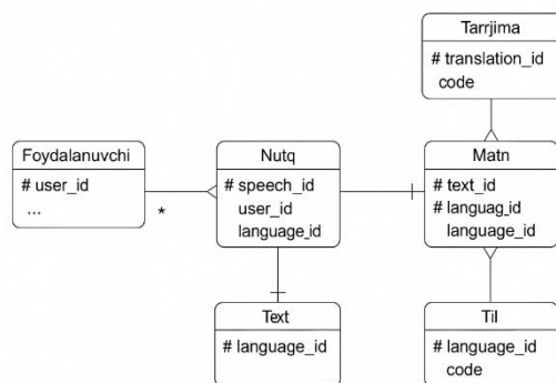
2-rasm. IDEF1X modeli.
